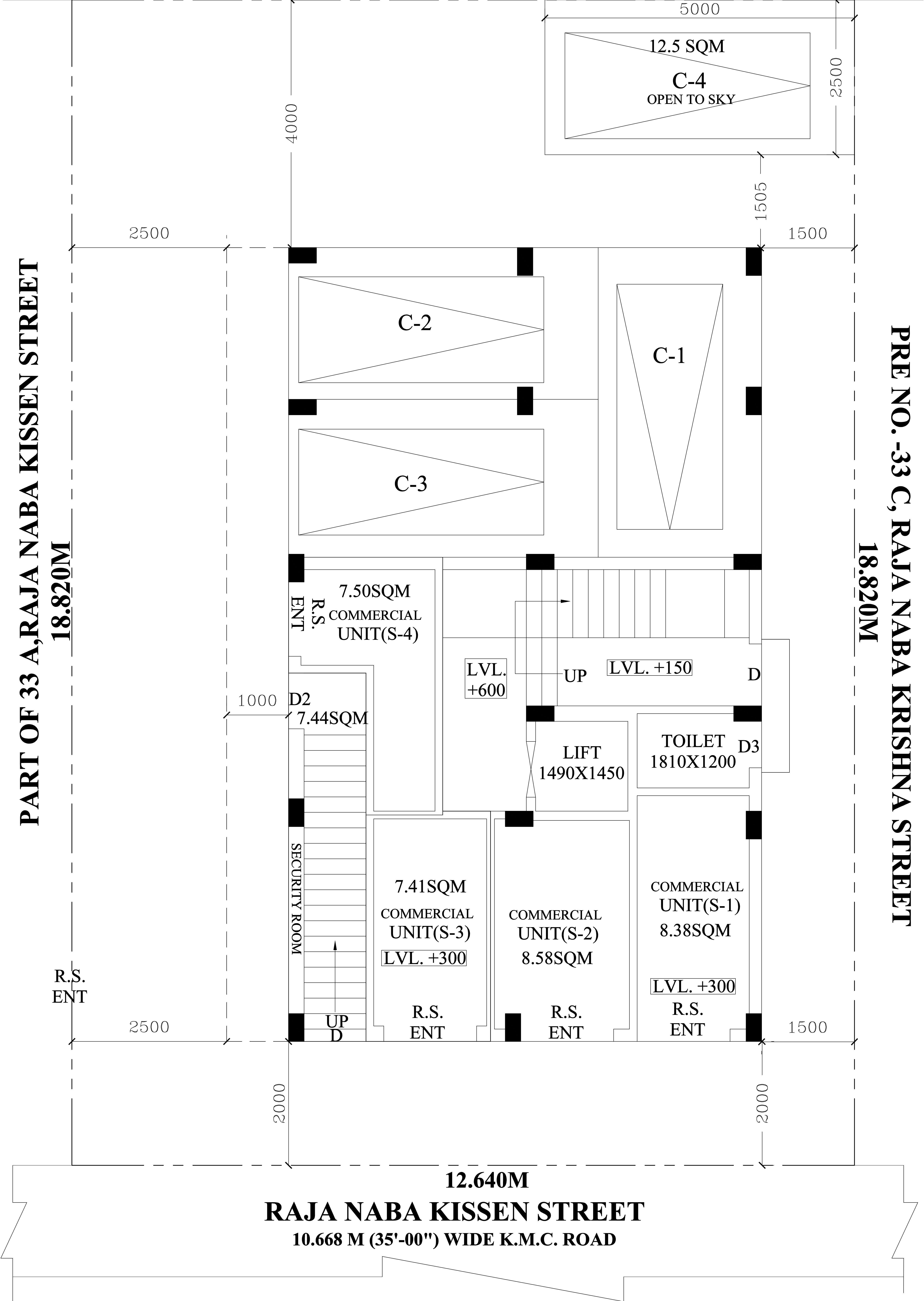
PROPOSED GROUND FLOOR PLAN SCALE:- 1:100
