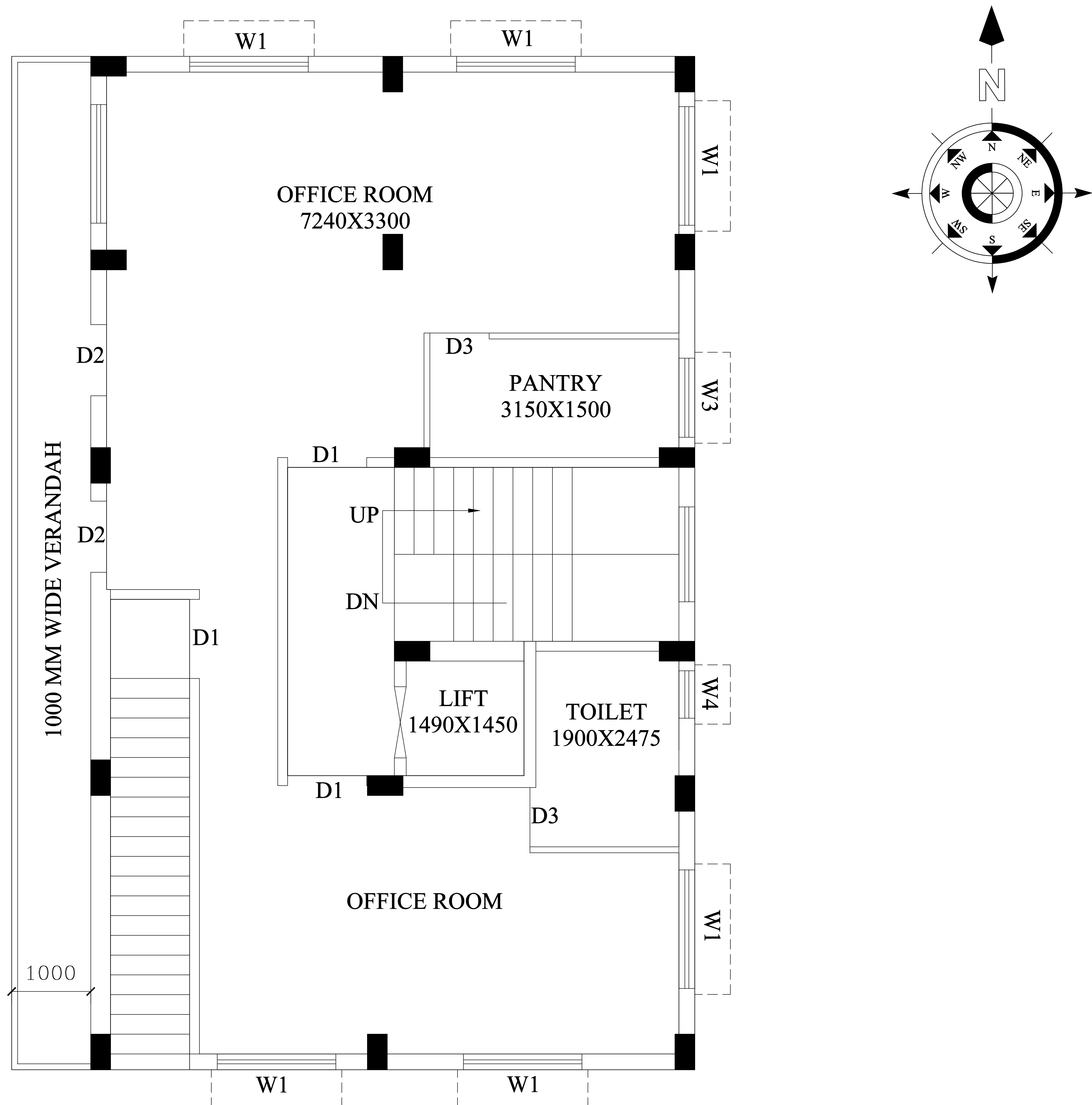
PROPOSED 1ST FLOOR PLAN SCALE:- 1:100
