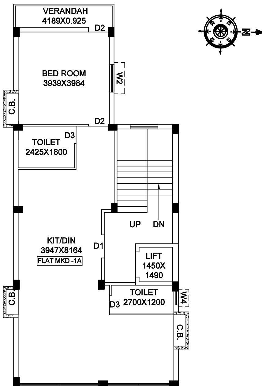
1ST FLOOR PLAN SCALE - 1:100
