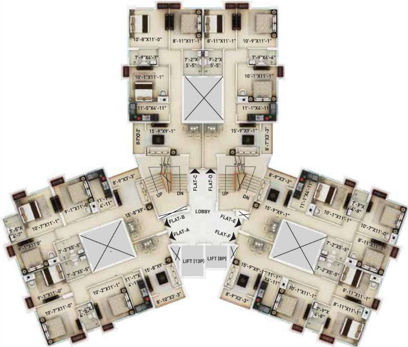
Block A Tower 1 (1 st to 14 th floor plan)
